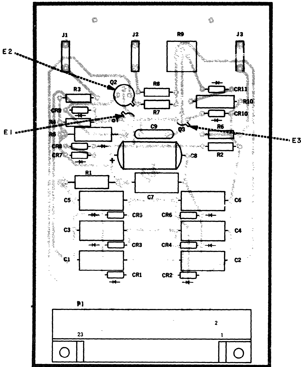
Figure 7 Filament supply, storage tube
