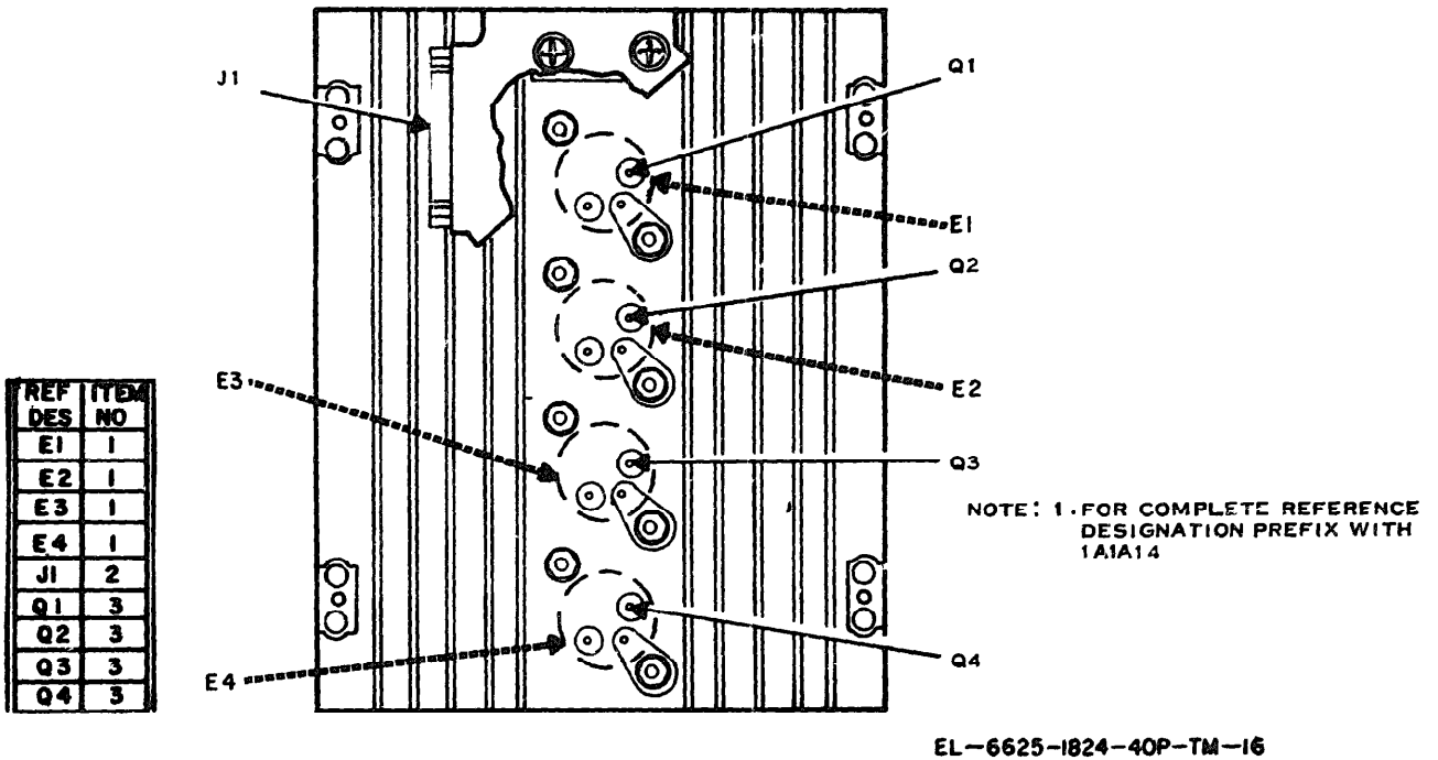
Figure 16. Assembly, heatsink 1A1A14
