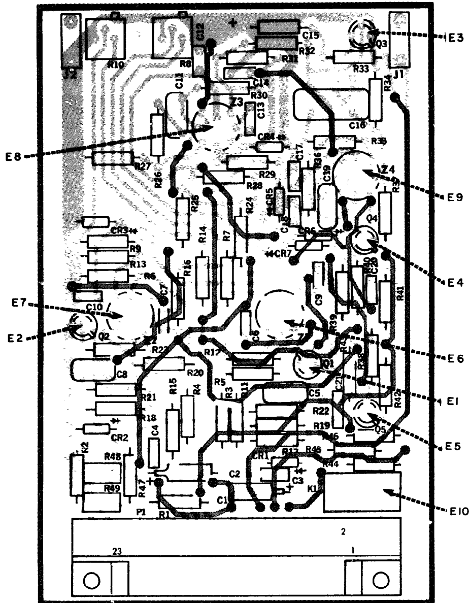
Figure 26. Amplifier, write video
