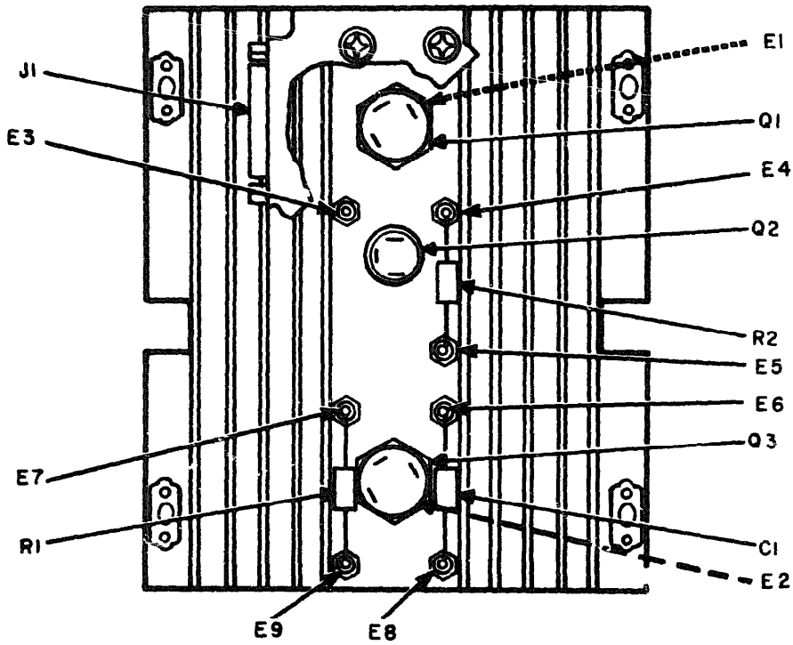
Figure 15. Assembly, heatsink IA1A13
