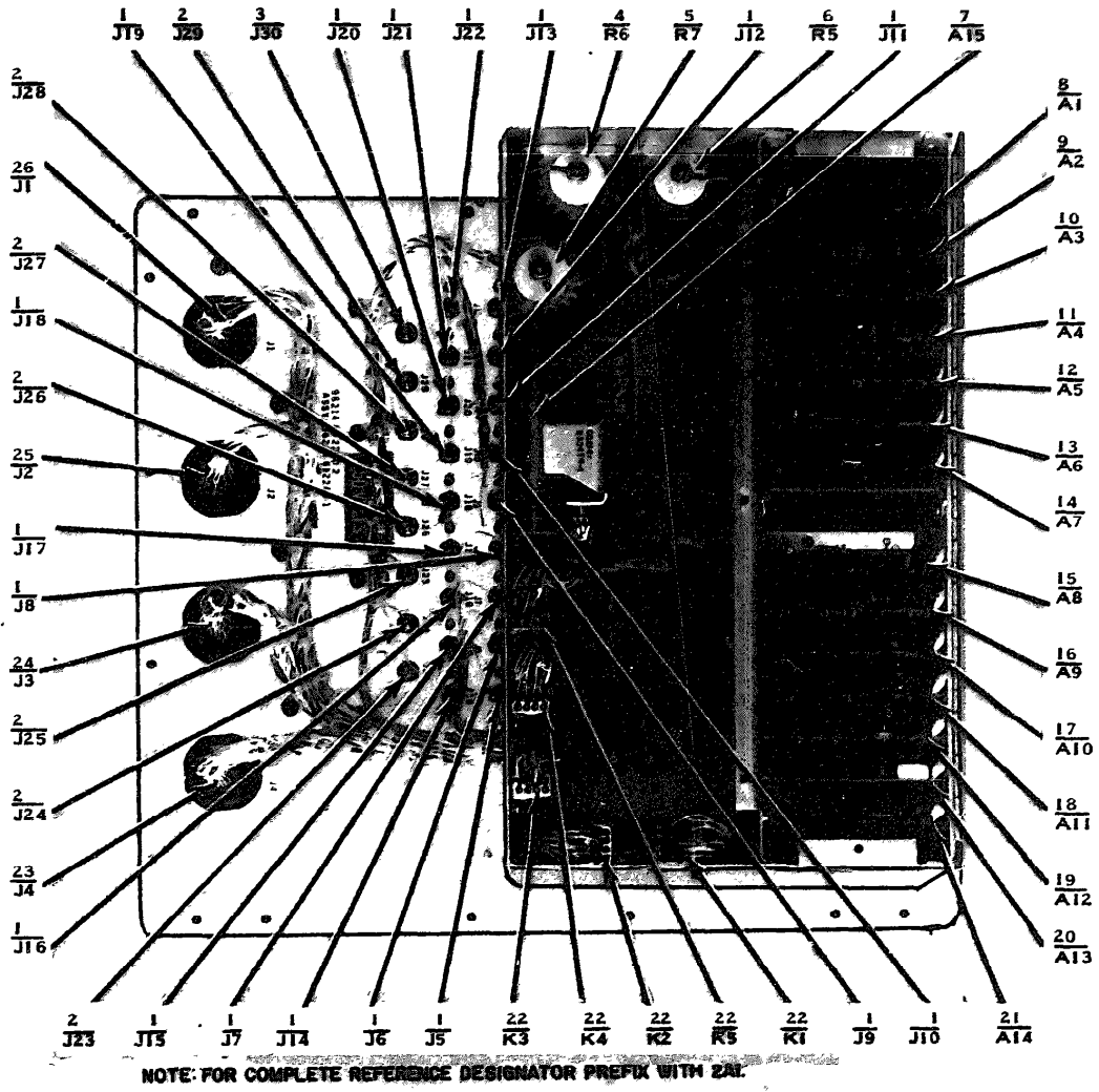
Figure 20-1. Control unit 2 (sheet 1 of 3)
