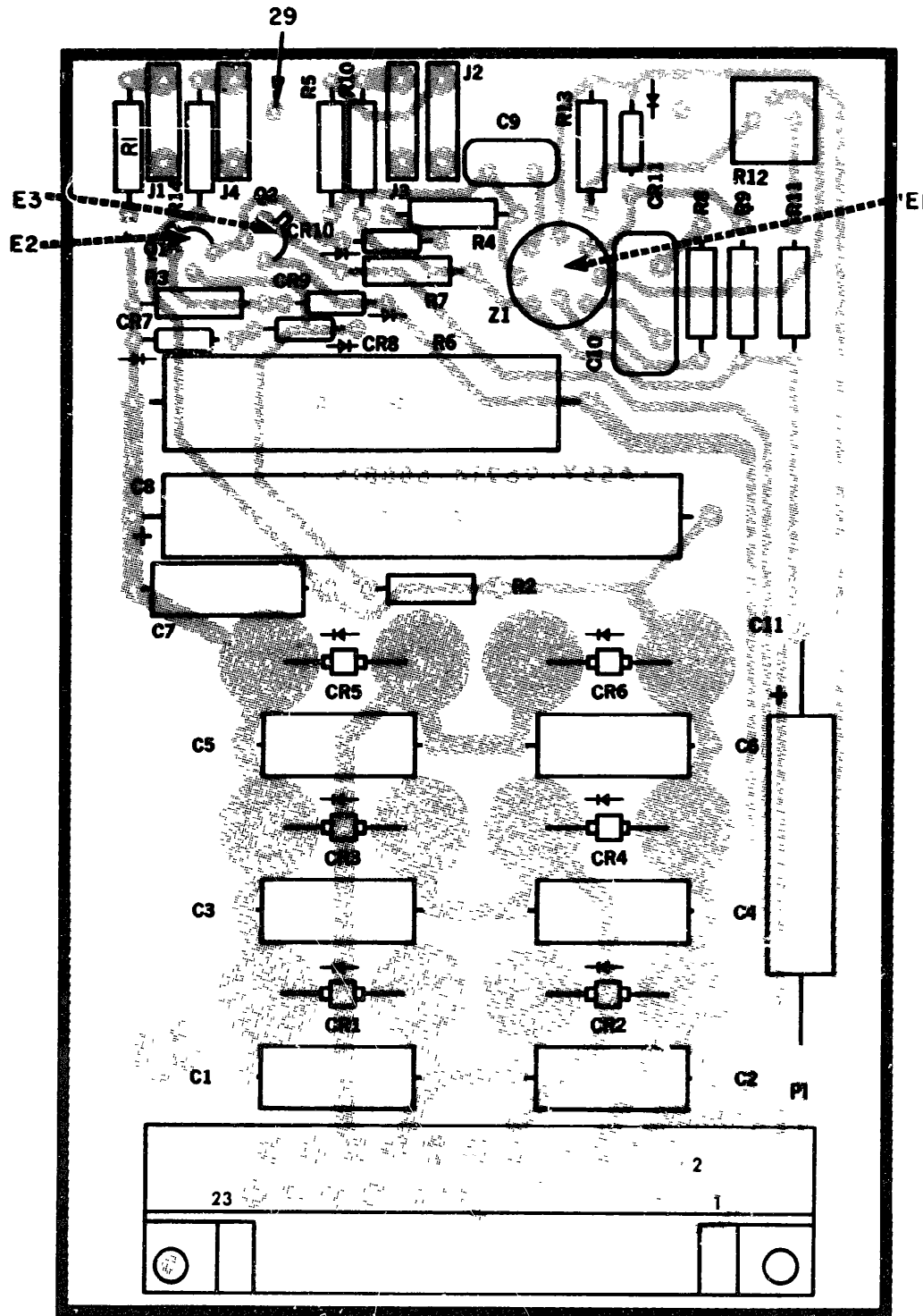
Figure 34. Power supply, +15 Vdc
