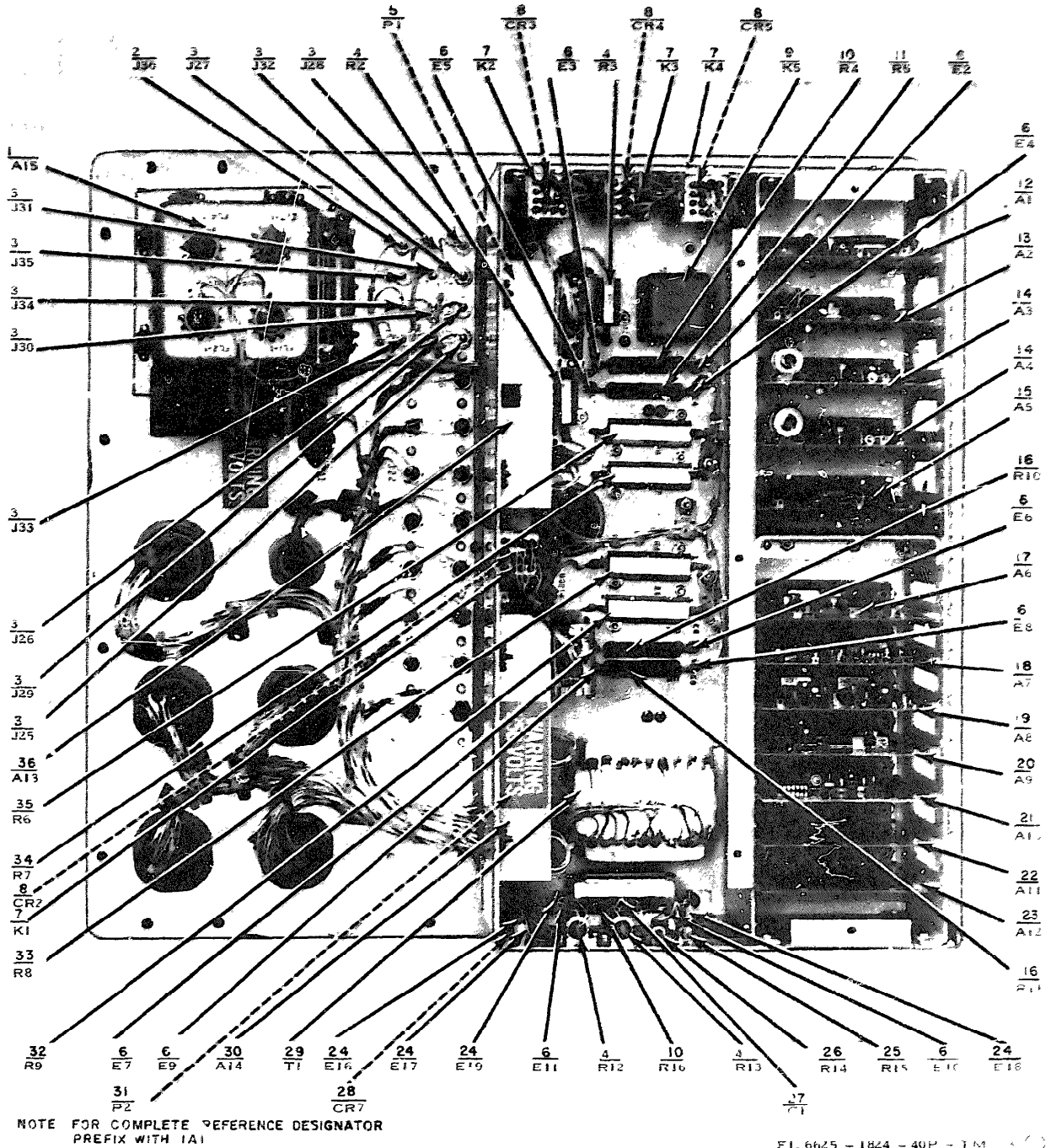
Figure 3 (1) Control unit No 1 (sheet 1 of 3)
