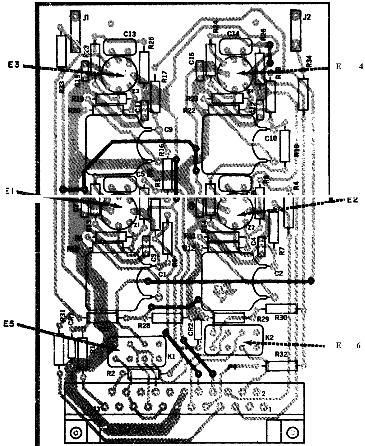
Figure 10. Video Interface
