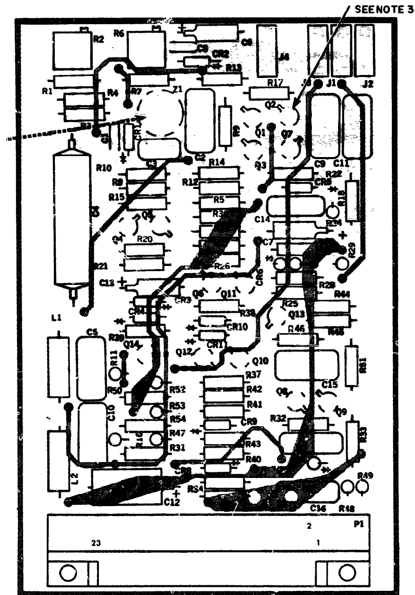
Figure 27 Generator, velocity/height clock pulse
