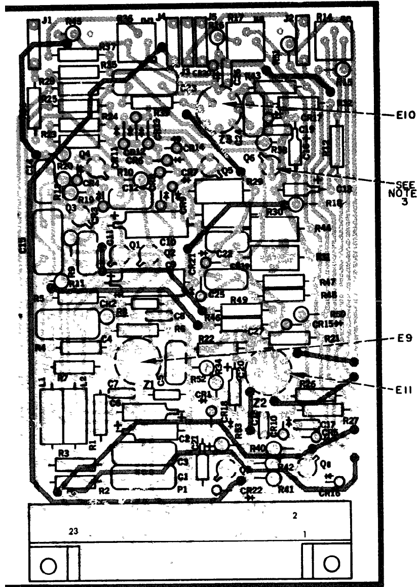
Figure 25 Slew, write horizontal and field-of-view adder
