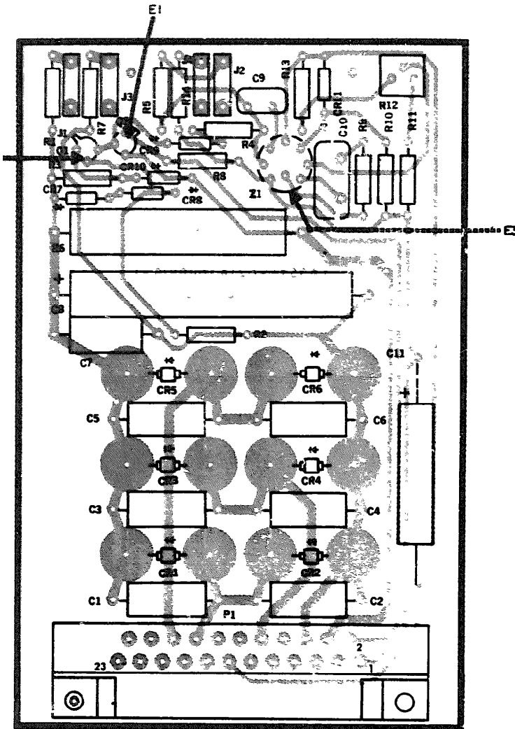
Figure 4 Power Supply - 15 VDC
