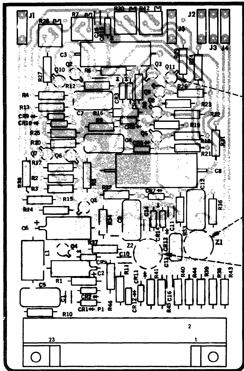
Figure 24 Generator, write horizontal sweep
