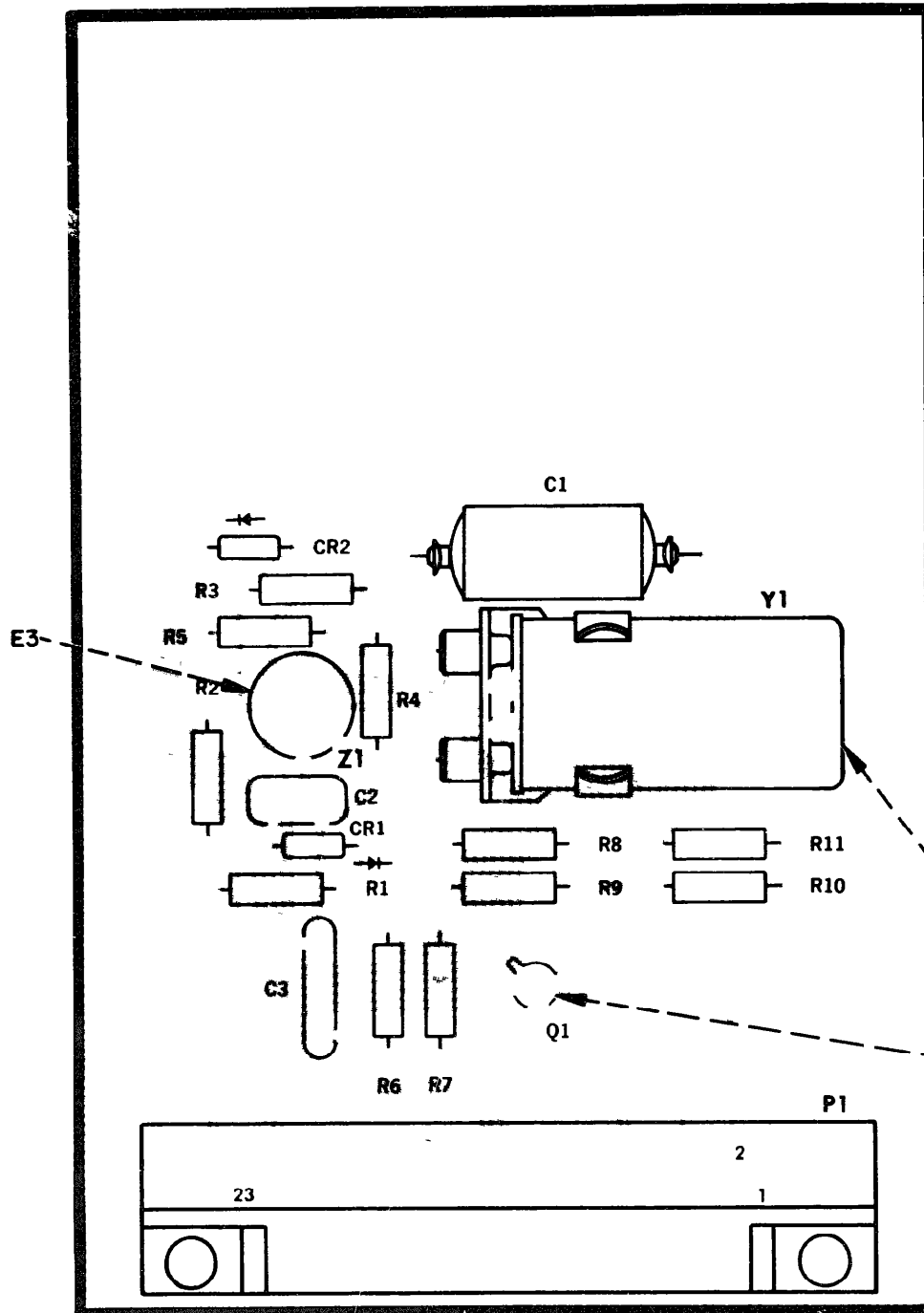
Figure 21 Oscillator, 100 kHz
